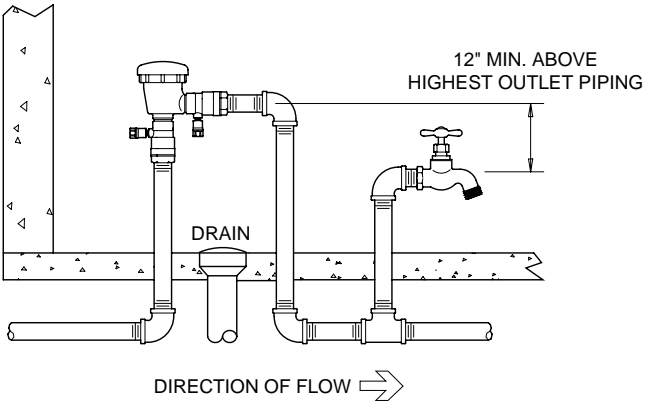
INDOOR INSTALLATION
