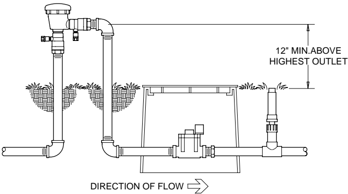
OUTDOOR INSTALLATION
