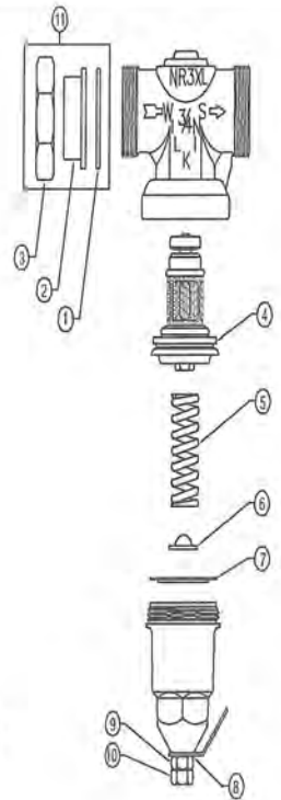
NR3XL (1/2", 3/4" & 1")
